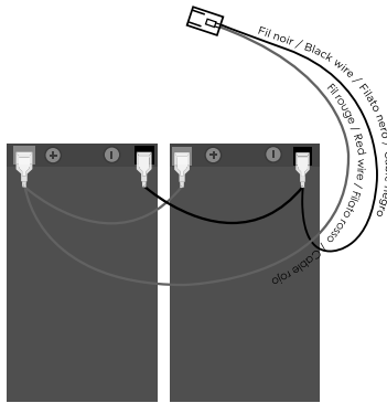
Branchement 12V sur séries OneGate (2017) 12V connection OneGate (2017) Cablaggio 12V OneGate (2017) Cableado 12V OneGate (2017)
