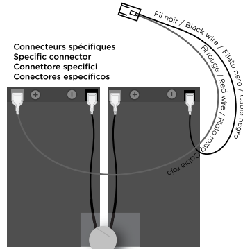
Branchement 24V sur séries PRO, HWAY, SCS, OPEN, OpenGate et SG à partir des versions 2016 24V connection ( PRO, HWAY, SCS, OPEN, OpenGate and SG from 2016 ranges) Cablaggio 24V ( PRO, HWAY, SCS, OPEN, OpenGate and SG a partire dalle versioni 2016) Cableado 24V ( PRO, HWAY, SCS, OPEN, OpenGate and SG a partir de las versiones 2016)
